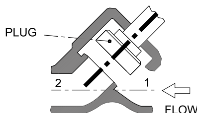
NORMALLY OPEN-FLOW TO CLOSE PLUG CAT. NO. 6622E / 6624E (FTC)
